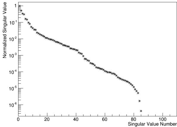
Figure 1: Singular values of the dispersion/corrector Jacobian. Note the large drops in singular value.
