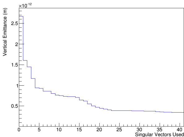
Figure 2: Vertical emittance as a function of singular vectors used to minimize it. Although we have 85 corrector magnets, only 10 combinations are needed to reduce the emittance by more than a factor of 3.
