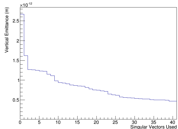
Figure 4: Vertical emittance as a function of modified singular vectors used to minimize it. We see improvements comparable to those in Fig. 2, when we made no attempt to minimize orbit changes.
