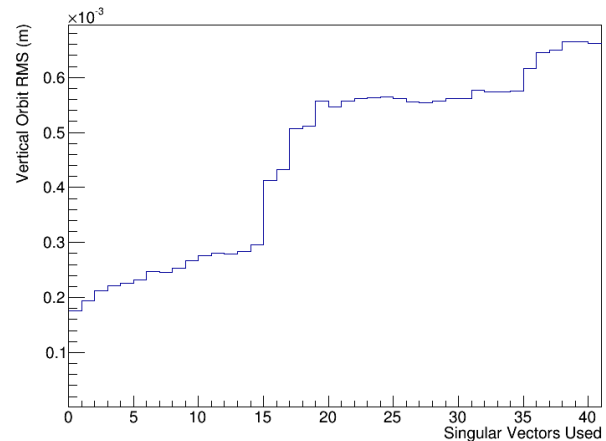
Figure 3: Vertical orbit RMS as a function of number of singular vectors used. We see an increase by nearly 100 microns if we use ten singular vectors, and 400 microns if we use 25.
