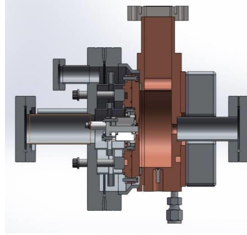
Figure 2: Engineering design of the cathode assembly test stand with indirectly cooled detachable back plate
