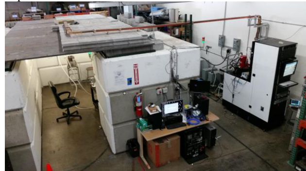
Figure 5: RadiaBeam radiation bunker. CPI klystron and magnetron modulator are on the right-hand side.
