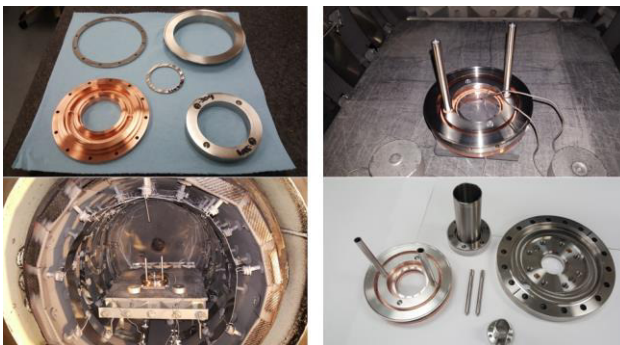
Figure 4: Various parts manufactured and brazed including cooling assembly piece parts (upper left), brazing assembly setup in the oven (upper right and lower left) and parts sent to welded bellows manufacturing vendor (lower right).
