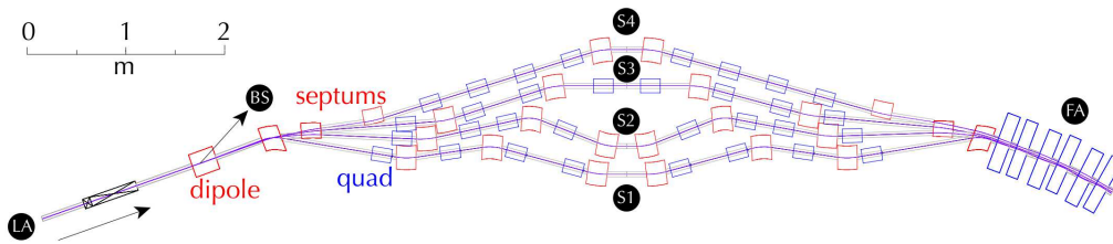
Figure 2: Layout of the splitter region
