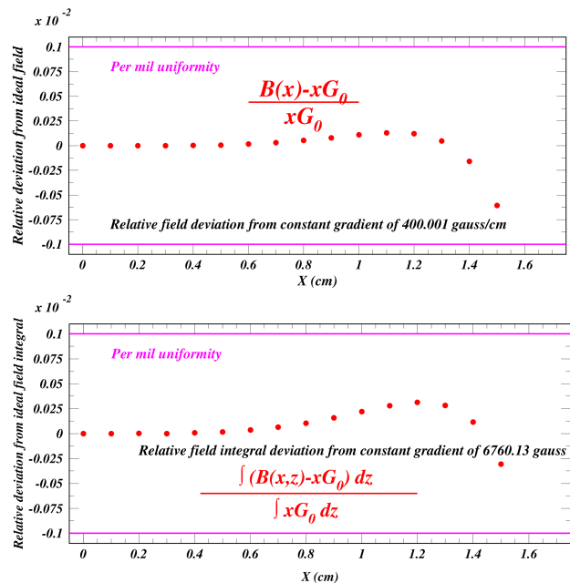
Figure 5: Uniformity of the 4.0 T/m quadrupole field. The upper plot shows the relative deviation of the field from a linear field with gradient equal to the central gradient at the longitudinal center of the magnet. The lower plot shows the relative deviation of the field integral from that of the perfectly uniform case. The 10 -3 specification is satisfied over 30 mm of the 34-mm width of the vacuum chamber.
