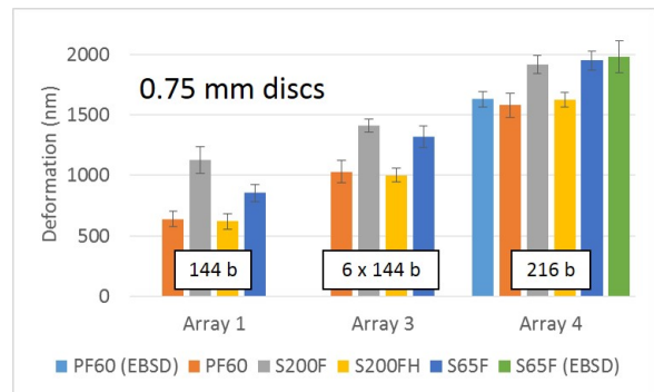
Figure 8: Out-of-plane deformations of 0.75 mm thick discs.
