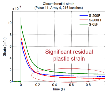
Figure 6: Strain response of slugs in Array 4 (216 bunches).
