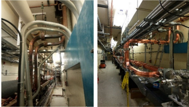
Figure 9: Old (left)/ new (right) waveguides.
