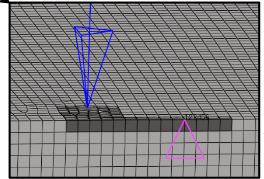
Fine 3D mesh
