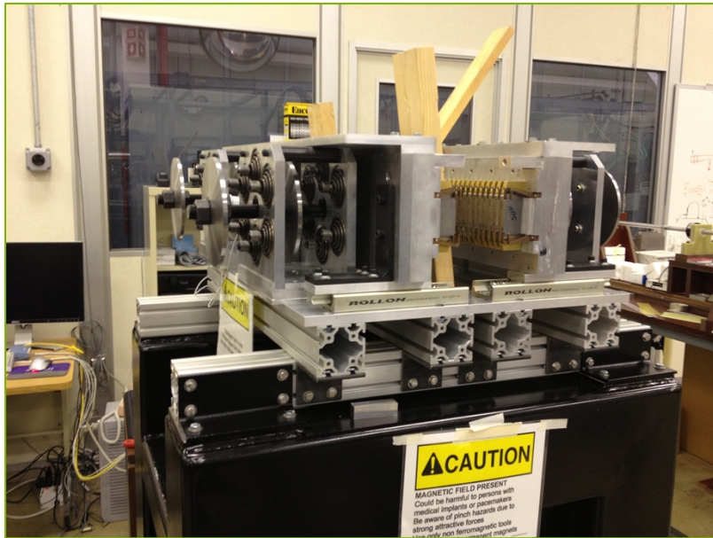
0.8 Meter-Long Prototype
