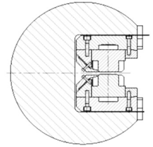
LCLS-I Cross-Section
