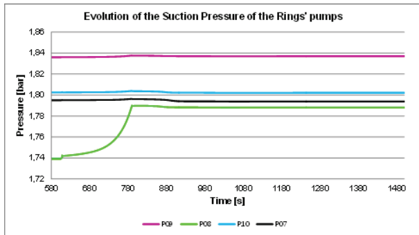
Figure 6: Pumps' suction pressures evolution during the SR's pipe blockage.
