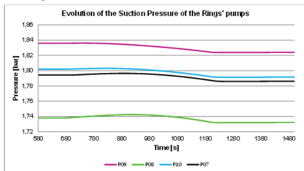
Figure 3: Pumps' suction pressures evolution during the SR's thermal load shut-down.
