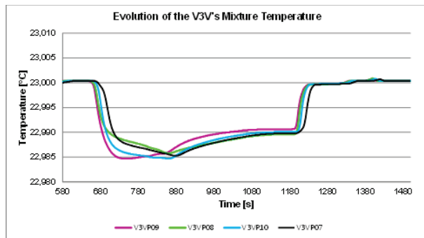
Figure 2: Temperature evolution due to the SR's thermal load shut-down.
