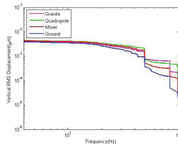
Figure 10: RMS Displacement spectra (vertical direction).
