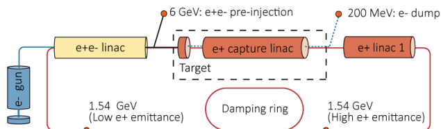
Figure 1: Latest proposal for the FCC-ee Injector Complex.
