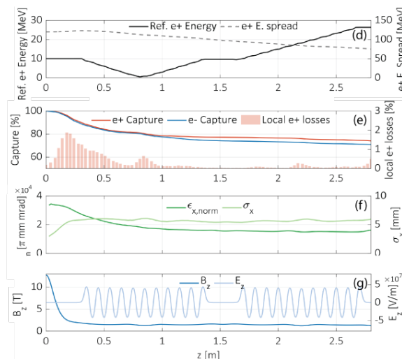
Figure 4: Longitudinal profile of P^3 beam at z = 2.85 m a to c) and evolution of main parameters (d to g).
