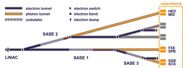
Figure 2: Arrangement of two hard x-ray undulators (SASE 1 und SASE 2), and a soft x-ray undulator (SASE 3) installed downstream of SASE 1.
