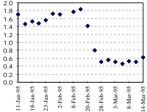
Chart 3, Losses during quadrupole retuning studies.
