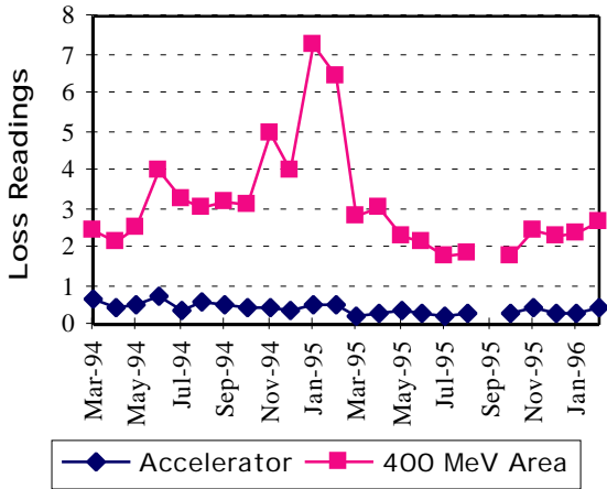
Chart 2, Average Losses.
