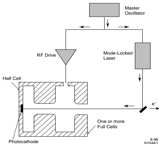
Fig. 1. Principal components of an rf photoinjector.
