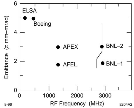
Fig. 2. Measured emittances scaled to 1 nC for a sample of emittance-compensated (except BNL-1) rf photoinjectors: ELSA,[19] Boeing,[20] APEX,[21] AFEL,[22] and BNL-1[23] The vertical range shown for BNL-2 corresponds to the estimate in reference 24.
