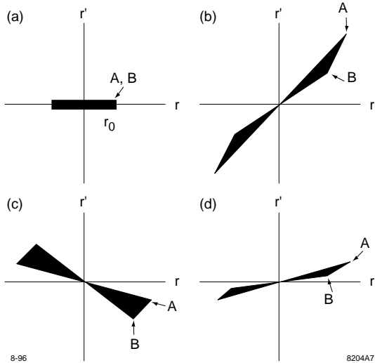
Fig. 4. Transverse phase-space plots: (a) initial conditions; (b) after drift to lens; (c) immediately after lens; and (d) after an additional drift behind lens.[25]
