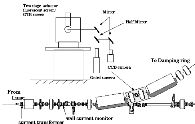
Fig. 1. Location of the OTR monitor for ATF linac.
