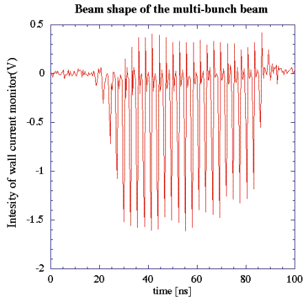
Fig. 5. Beam shape of the multi-bunch by the wall current monitor at the end of the ATF linac.
