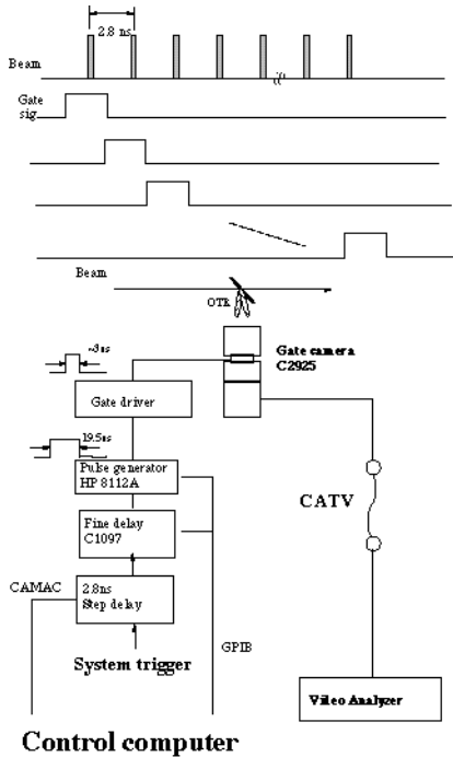
Fig. 2. Trigger system of the gate camera.
