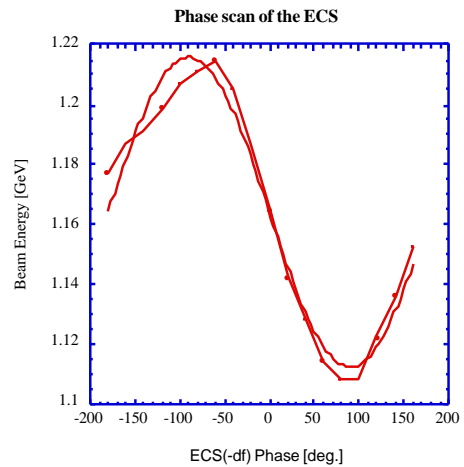
Fig. 4. Phase scan of the compensation section.
