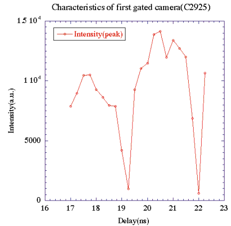
Fig. 3. Gate characteristics of the gate camera.
