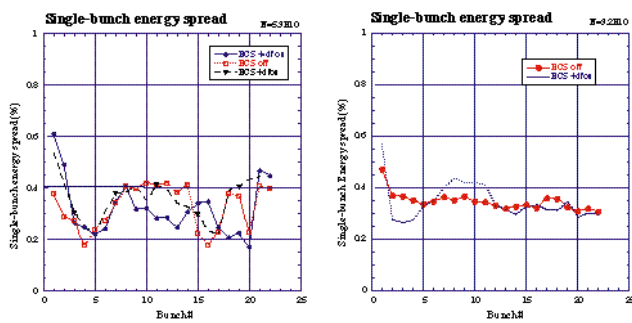
Fig. 7. Single-bunch energy spread: a) total charge/pulse = 5.3 \times 10^{10} , b) total charge/pulse = 3.2 \times 10^{10} .
