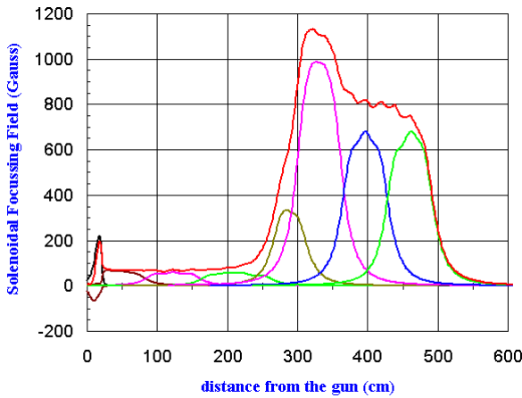
Figure 2. Solenoidal focusing fields are constructed by linear superposition of individual solenoid fields.
