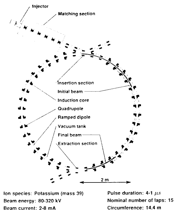
Figure 4. Diagram of recirculator experiment.
