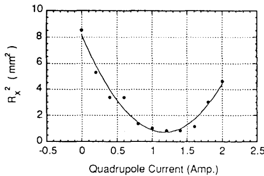
Fig. 7 Squared beam radius vs. Q-mag strength.
