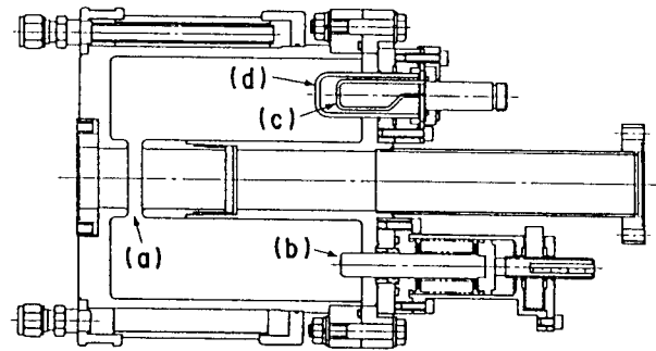
Fig. 2 SHB cavity: (a) Acceleration gap, (b) tuner, (c) coupler, and (d) ceramic window.
