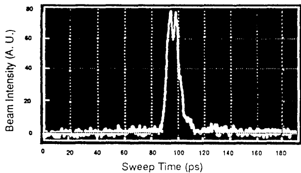
Fig. 4 Main bunch structure of a 6-nC beam.
