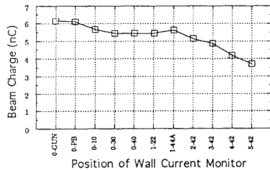
Fig. 6 Single-bunch beam accelerated in the PF linac.
