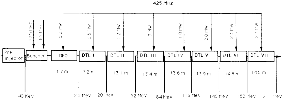
Figure 1: Block diagram of the Linac
