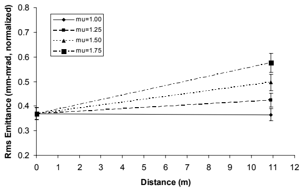
Figure 5: Simulation results for the average transverse rms emittance at the entrance and exit of the beam line for the breathing mode at 75 mA.
