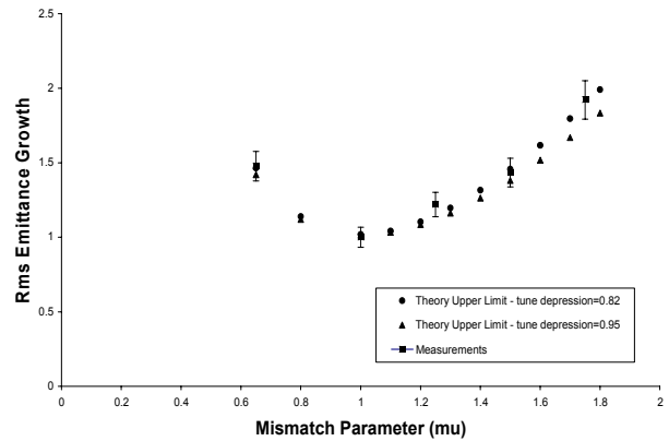
Figure 6: Rms-emittance growth, averaged over x and y, at scanner 20, 75mA, breathing mode.
