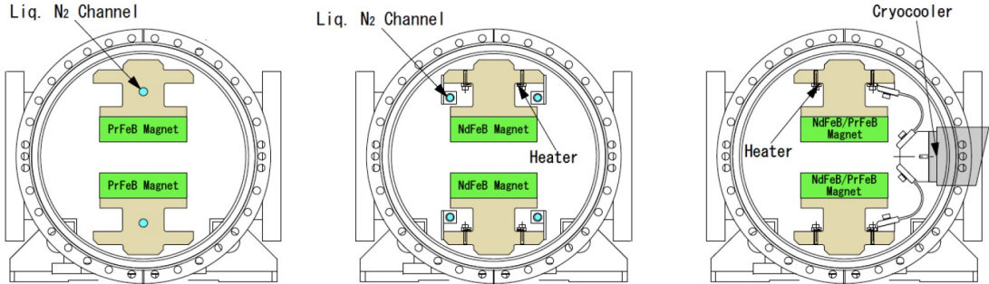
(a) Direct cooling of PMs with LN 2 , (b) indirect cooling of PMs with LN 2 and temperature control, (c) indirect cooling of PMs with cold head and temperature control
