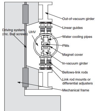
In-Vacuum Undulator
