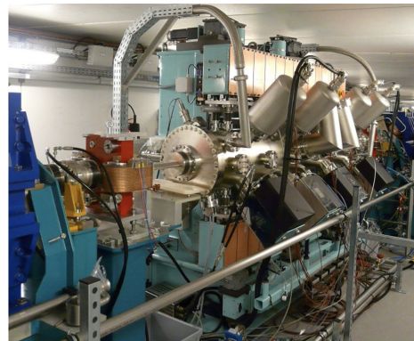
Installation of a Cryogenically Cooled In-Vac at Soleil
