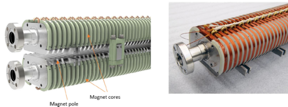
Fig. 9. Rendering and picture of APS SCU magnet core.
