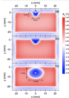
Demagnetization, or field reversal, in a SACLA in-vacuum undulator [8]
