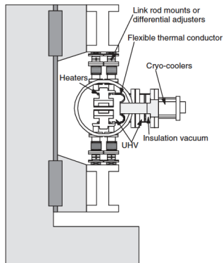
Cryogenic Permanent Magnet Undulator for TPS
