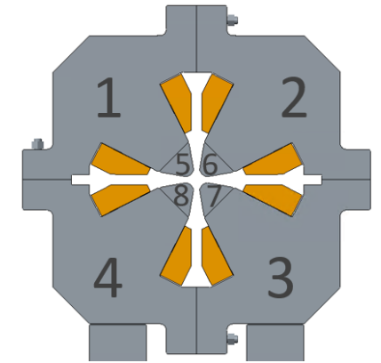
Magnet Yoke
