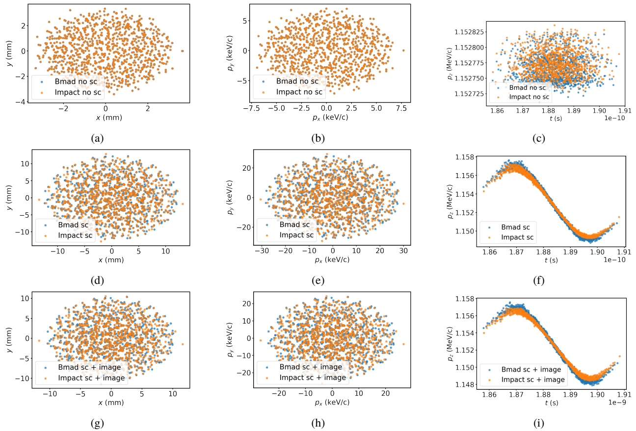
Figure 4: Phase space comparison at the end of a DC gun between Bmad and Impact-T. (4a,4b,4c) No space charge effect. (4d,4e,4f) With space charge. (4g,4h,4i) With space charge and image charge.
