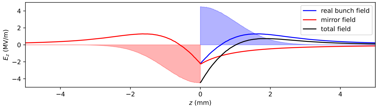
Figure 1: Space charge field for a Gaussian bunch and its image charges near the cathode at z=0 . Left axis is the field strength and right axis is the charge density. The space charge field pushes particles in the head of the bunch forward and particles in the tail backward. The image field attracts the bunch towards the cathode surface, the effect of which is important close to the cathode.
