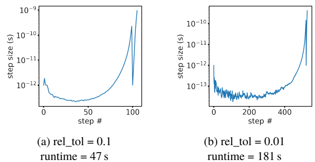
Figure 3: Time steps taken by adaptive step size control under two tolerance settings and their runtime. abs\_tol = 10^{-6} in both (a) and (b).
