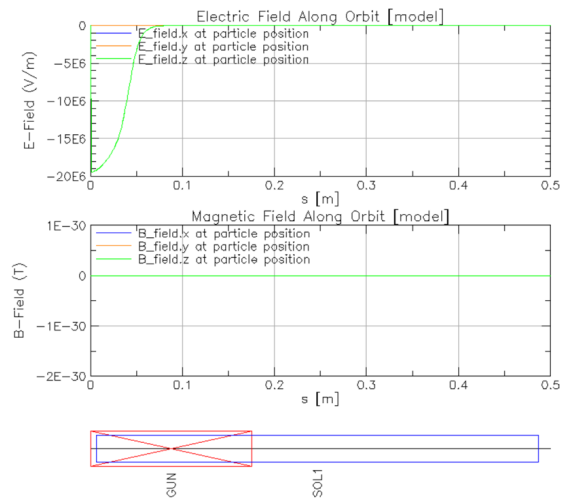
Figure 2: A lattice of a 750 kV DC gun is used for validation of cathode space charge tracking. The solenoid is turned off.
