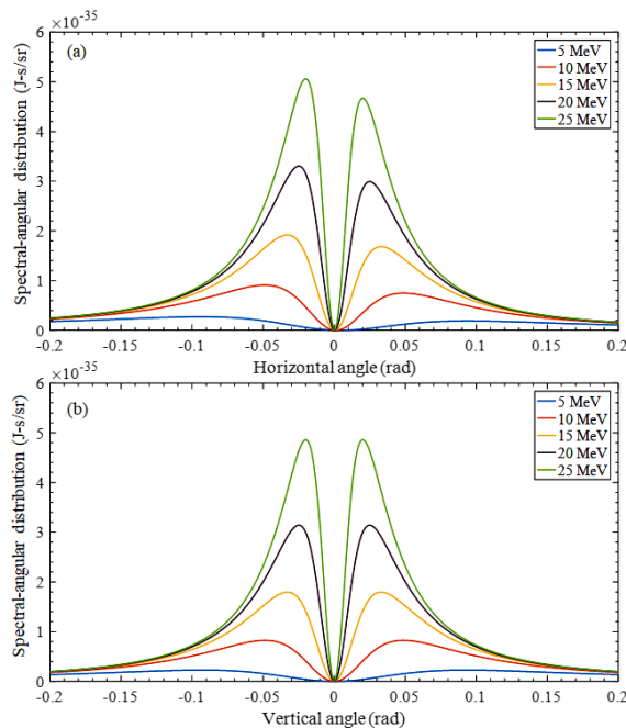
Figure 2: Backward angular distributions of TR for various electron energies with (a) horizontal cross section and (b) vertical cross section.
