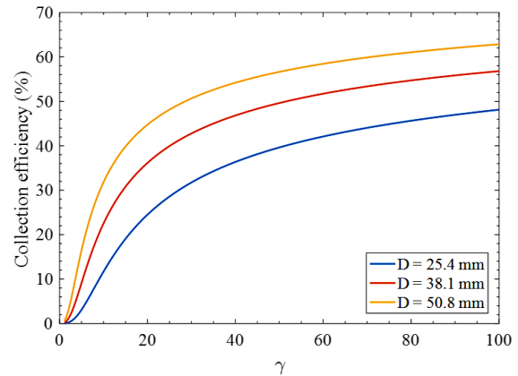
Figure 3: Collection efficiency of transition radiation as a function of electron beam energy ( \gamma ) with different parabolic mirror diameter ( D ).
