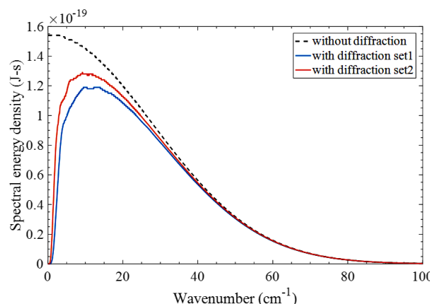
Figure 6: Coherent transition radiation spectra showing the effect of mirror diffraction for electron beam with energy of 10 MeV and bunch length of 40 \mu\text{m} .
