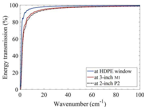
Figure 5: Energy transmission through the setup with improved design (set 2) versus the radiation wavenumber.
