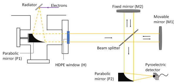
Figure 1: The setup for backward CTR generation and Michelson interferometer for radiation spectrum measurement.
