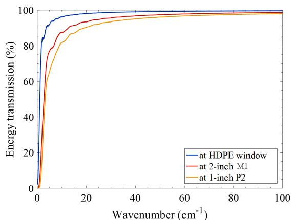
Figure 4: Energy transmission through the original setup (set 1) versus the radiation wavenumber.
