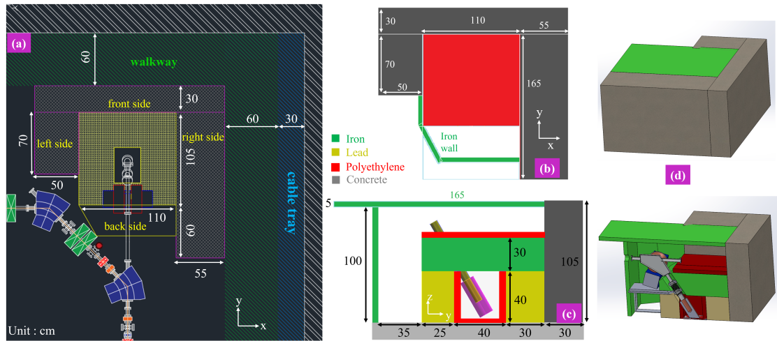
Figure 2: (a) The sketch of the beam dump No.1 and its local shielding with the surrounding area. (b) Top view and (c) side view of the final model of the shielding. (d) The 3D model of local shielding for the beam dump No.1 (top) and the model with cutting plane at center of the beam dump (bottom) [1].
