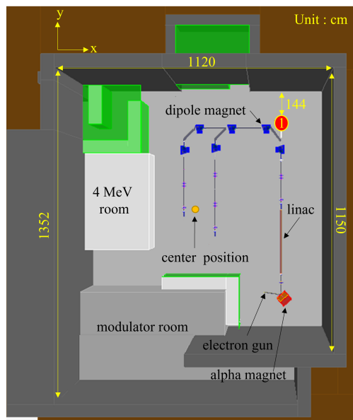
Figure 1: The top view of GEANT4 3D drawing of the PCELL accelerator hall based on the actual dimension. The linear accelerator (linac) can be seen as a red pipe housed inside the hall. The red circle with number 1 marks the position where the electron beam is dumped into a Faraday cup [1].
