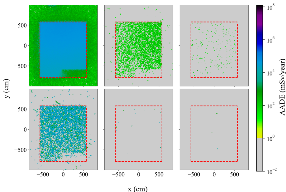
Figure 3: AADE maps of photon (top) and neutron (bottom) at the roof of the accelerator hall, in the case of without shielding (left), adding the first barriers (center), and final model of shielding (right).
