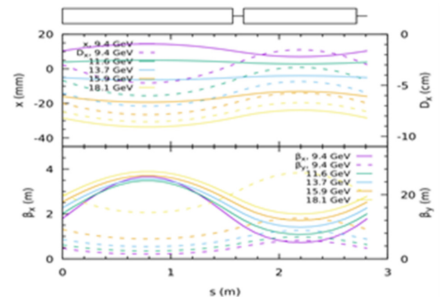
Figure 4: Orbital offset (top, left scale), dispersion (top, right scale) and horizontal (bottom, left scale) and vertical (bottom, right scale) Twiss \beta functions of a regular periodic cell of the FFA 1 west arc.
