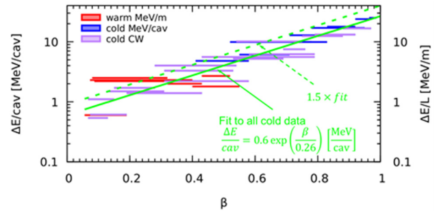
Figure 1: Summary of the energy gains per cavity versus the cavity's velocity range for the seven selected projects. The warm linac data is shown in red on the right vertical scale in terms of the energy gain per unit length.
