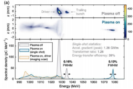
Figure 1: Preservation of the energy spread and the high efficiency acceleration based on strong beam loading induced by peculiar charge density profiles [7].
