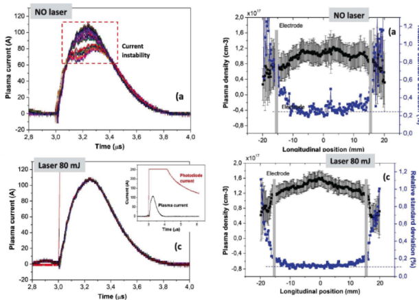
Figure 4: Current profiles (left) and plasma density (right) measured without (top) and with (bottom) pre-ionization laser.
