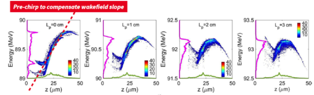
Figure 2: Witness beam longitudinal phase space: minimization of energy spread based on assisted beam loading technique [8].
