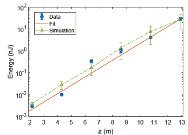
Figure 3: Exponential gain of SASE FEL radiation energy at SPARC_LAB. Data are taken with six (Si) photo-diodes downstream the undulators.
