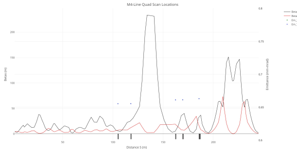
Figure 3: Tracking the beta functions along the muon campus extraction line. The dots represent the location and the emittance of the five quads that were scanned. The black rectangles at the bottom of the figure represent the relative size and location of the quadrupole magnets.
