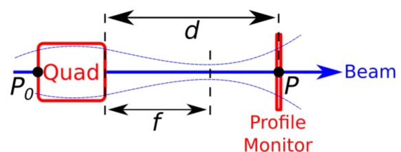
Figure 2: Visual representation showing the principle of the quad scan technique.
