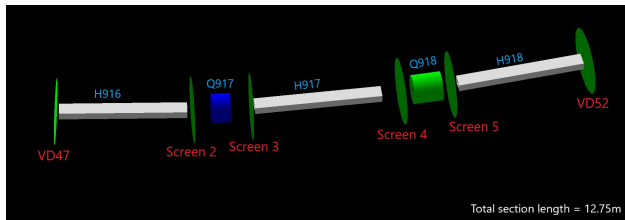
Figure 7: Simulated test section for the 6-screen-method. "VDs" and "screens" are simulated profile monitors. The long grey rectangles are dipoles and the cylinders are quadrupole magnets.
