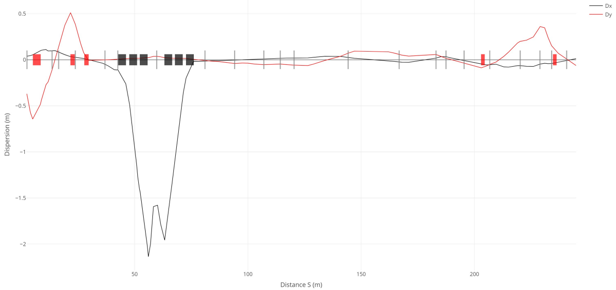
Figure 6: This plot tracks the dispersion along the Muon Campus extraction line. The red rectangles represent vertically bending dipoles, the black rectangles represent horizontally bending dipoles and the grey lines represent profile monitors.
