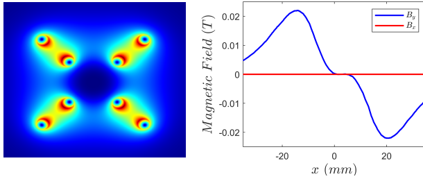
Figure 1: NLK preliminary design 8 conductor configuration and the nonlinear magnetic field B_y .
