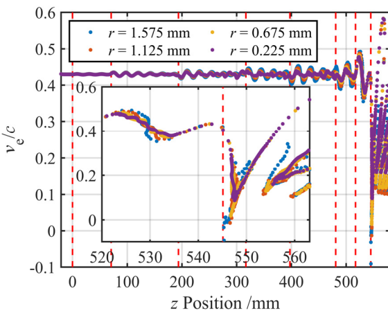
Figure 7: Electron velocity trajectories at different radii calculated by KlyC/1.5-D.
