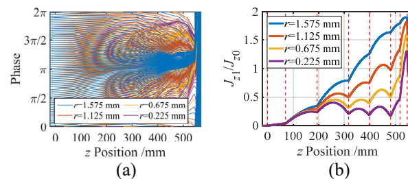
Figure 3: Phase trajectories and the first order current harmonics at different radii calculated by KlyC/1.5-D.
