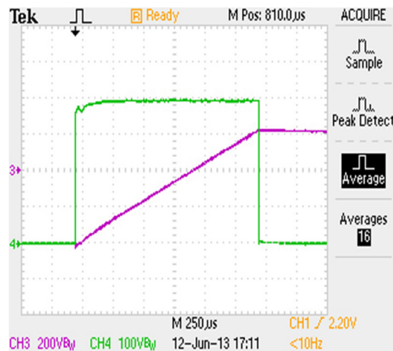
Figure 4: Pulse voltage (green) and regulator voltage (purple) with the regulator, 200 V/div, 250 \mu s/div.
