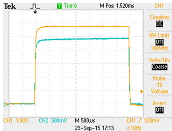
Figure 2: Voltage and current waveforms of the ESS modulator.
