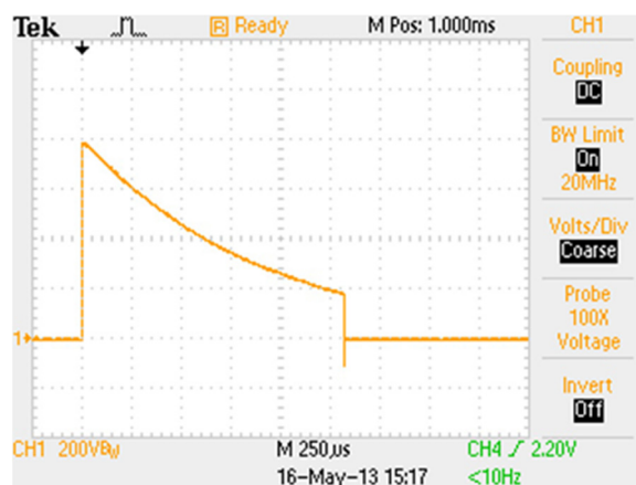
Figure 3: Pulse voltage without the regulator, 200 V/div, 250 \mu s/div.
