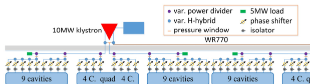
Figure 1: PDS for ILC in ILC TDR [1].
