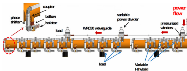
Figure 2: LPDS for ILC in ILC TDR [1].
