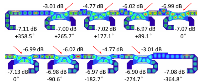
Figure 11: Simulation of compact LPDS.
