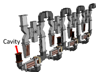
Figure 3: LPDS in the STF.
