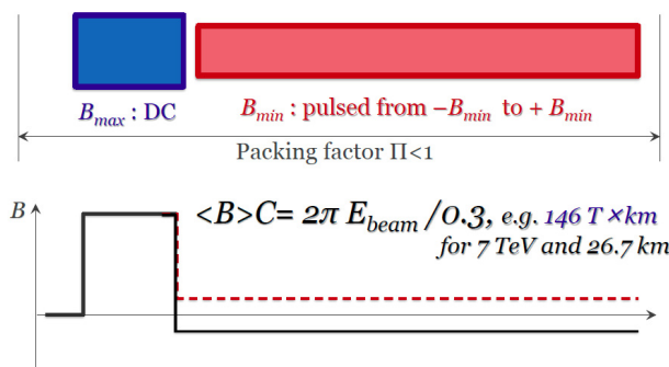
Figure 2: Arrangement (top) and field strengths (bottom) in the SC and pulsed magnets of the pulsed muon RCS.
