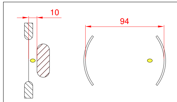
Figure 1: Cross-section of the booster injection septum and kicker.
