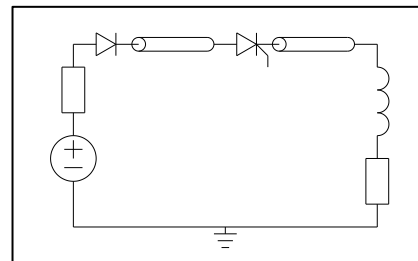
Figure 6: Schematic circuit diagram of the extraction kicker.
