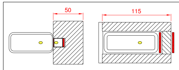
Figure7: Cross-section storage-ring injection septum and kicker.
