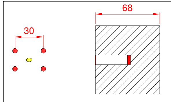
Figure 5: Cross-section of booster extraction septum and kicker.
