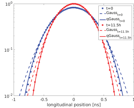
Figure 3: The initial ( t = 0 ) and the final ( t = 11.5 h) longitudinal bunch profiles, as calculated by SIRE, are denoted by blue and red stars respectively. They are fitted with the Gaussian (dashed line) and the q-Gaussian (solid line) functions.
