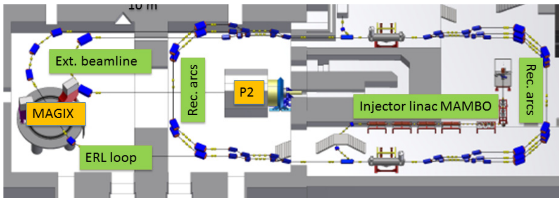
Figure 1: Layout of the MESA accelerator and planned main experiments MAGIX and P2.
