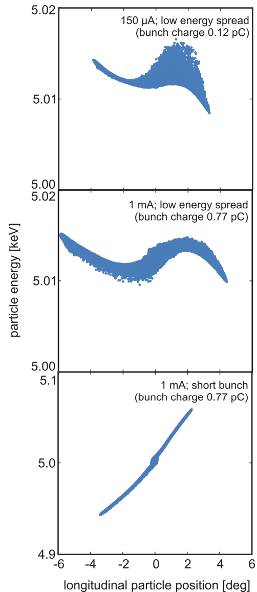
Figure 2: Simulated longitudinal particle distributions at the end of the MAMBO injector for different beam currents and optimized for different operating conditions. The RMS bunch length and energy spread is listed in Table 1.
