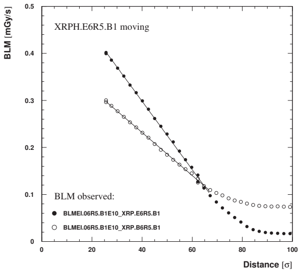
Figure 3: Dose rate at two BLMs, extrapolated to \mathcal{L} = 10^{34} \text{ cm}^{-2} \text{ s}^{-1} , as a function of the insertion distance of the XRPHE6R5 unit. For this study all other RPs are in retracted position.
