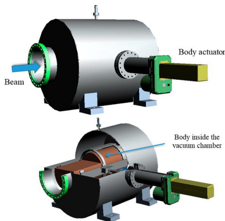
Figure 5: Faraday cup with longitudinally sectioned body.
