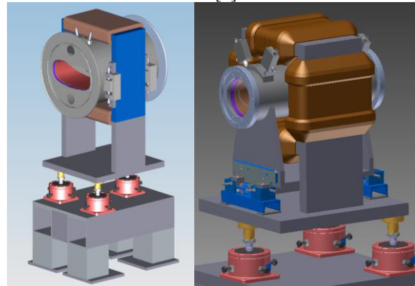
Figure 2: BPM installed in vertical (left) and combined (right) dipole corrector.
