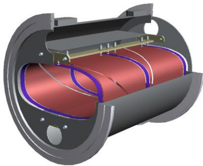
Figure 1: A large (400 mm) aperture, super-elliptical, split plate BPM design in dispersive section provides a larger linear response aperture.
