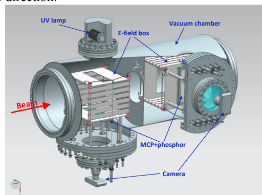
Figure 3: Combined RGM and its components.
