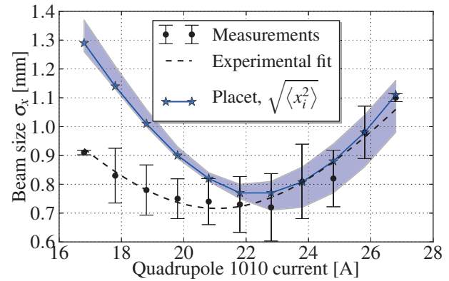
(b) Uncombined beam, 7 % deceleration.
