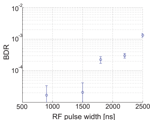
Figure 4: BDR as a function of the pulse width at 15 MW for the horizontal deflector.
