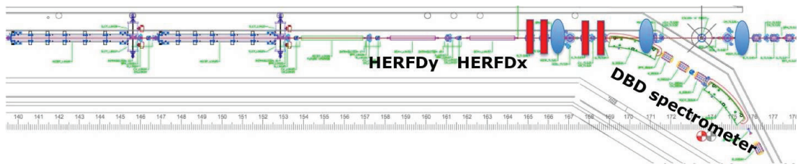
Figure 1: Layout of the end of linac, with the two RF deflectors, HERFDy and HERFDx.
