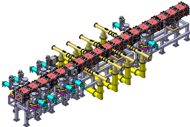
Figure 2: 3D mock-up of the RFQ equipped with RF couplers, cryo-pumps, slug tuners and cooling channels.
