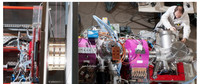
Figure 1: Top view of the Injector (P. Stroppa/cea credit).
