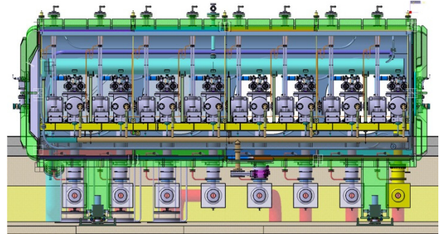
Figure 3: 3D mock-up of the LIPAc Cryomodule.
