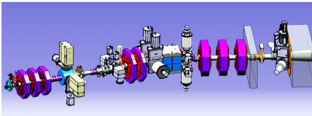
Figure 4: High Energy Beam Transport line.
