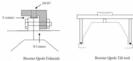
Figure 4: Booster quadrupole fiducials.
