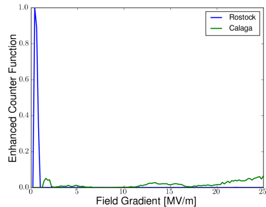
Figure 7: Comparison of the behaviour of the two couplers after normalisation by the total charge emitted during the simulation.
