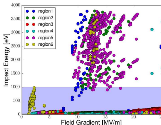
Figure 3: Impact energy of each electron vs the gradient of the accelerating field within the cavity.
