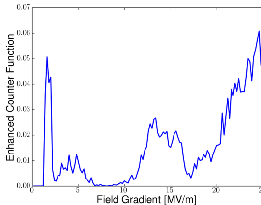
Figure 4: “Enhanced counter function” for Tesla-style design.
