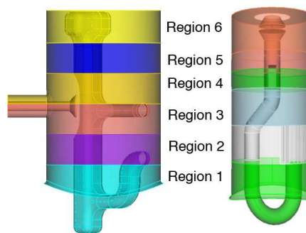
Figure 2: Left, Geometry of a coupler design generated by rescaling of a TESLA-style coupler. Right, Geometry of the alternative design. The regions indicated relate to simulation domains used in their analysis.
