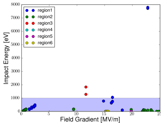
Figure 5: Impact energy of each electron vs the gradient of the accelerating field within the cavity.
