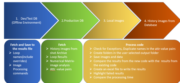
Figure 14: Flow of the IDL Code Analyzer testing tool process.
