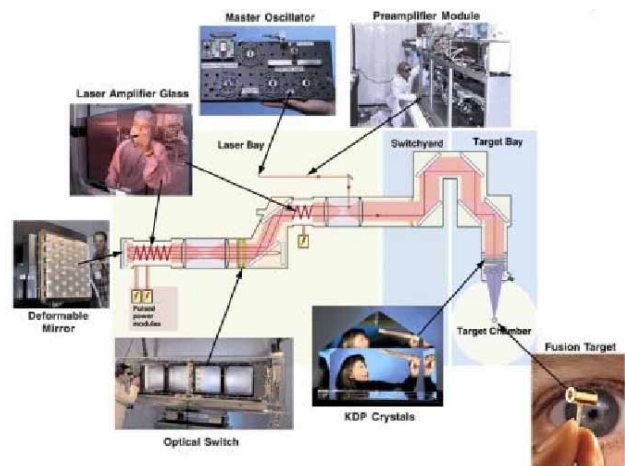
Figure 2: Schematic representation of a NIF laser beam line highlighting some of the key technologies.
