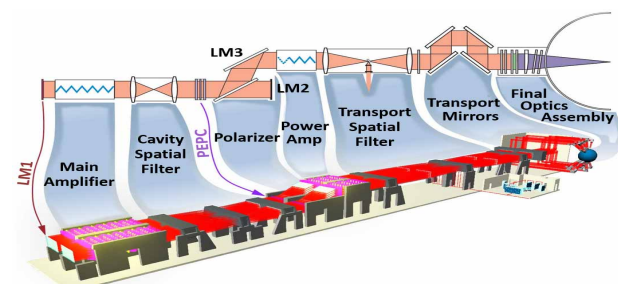
Figure 7: Main laser schematic of a single laser beam.
