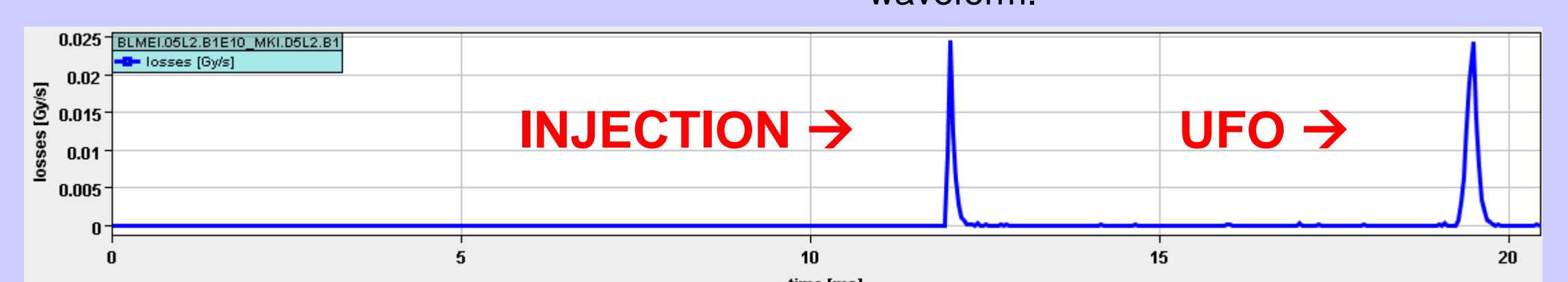
UFOs appear more frequently around the MKI at injection. In the IQC BLM plot they can be studied if they appear within the 20ms buffer.
