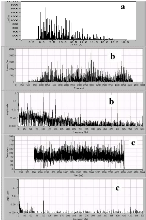
Figure 5: Beam spill structure and FFT results. (a) feedback off and RF-KO with constant RF power, (b) feedback off and RF-KO with amplitude changing, (c) feedback on and RF-KO with amplitude changing. Sample rate is 1KS/s. (200MeV/ \mu ^{12}\text{C}^{6+} )
