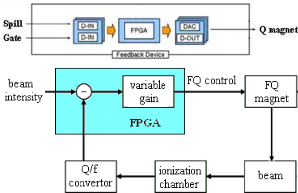
Figure 3: The spill feedback processing
