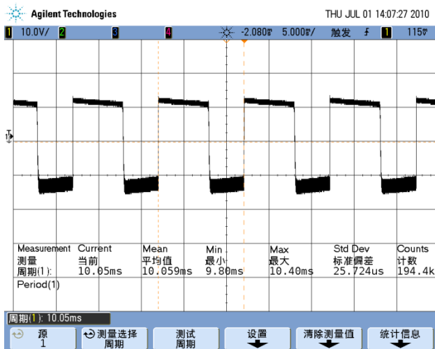
Figure 10: Jitter of 10ms period.
