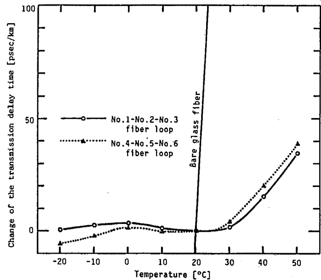
Fig.3 Temperature dependence of the transmission delay time
