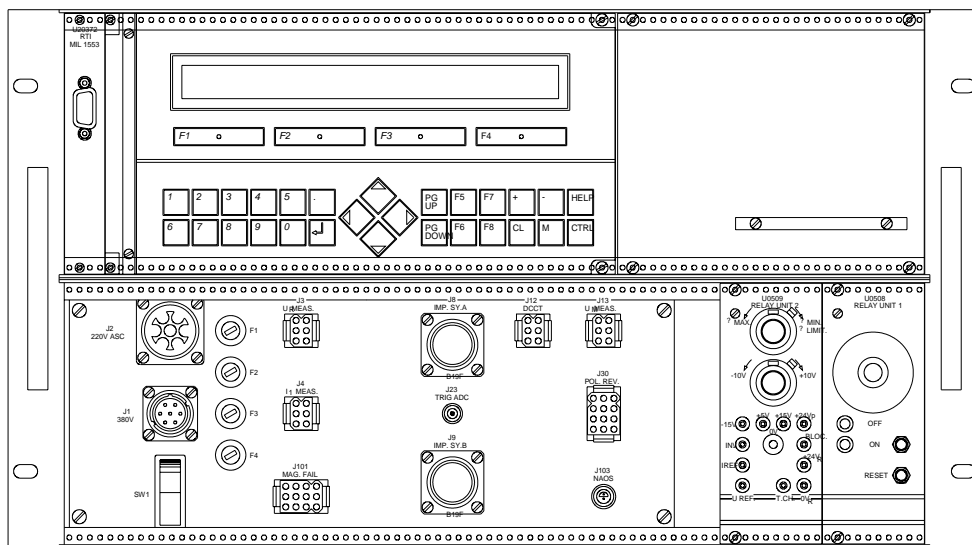
Figure 1: Front view of a CERN G-64 chassis
