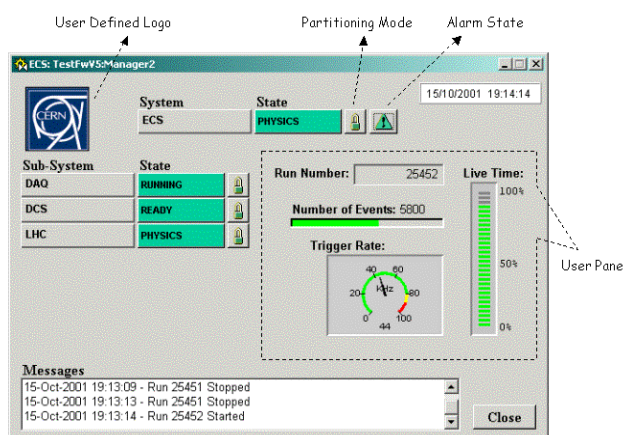
Fig. 4. Generic system operation interface
