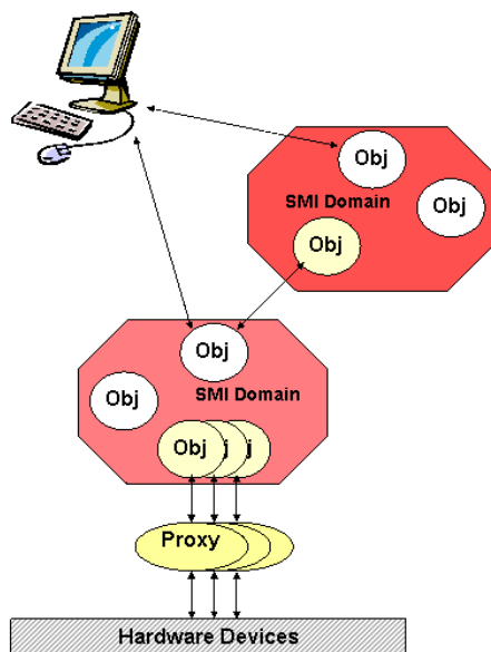
Fig. 2. SMI++ Run-time Environment
