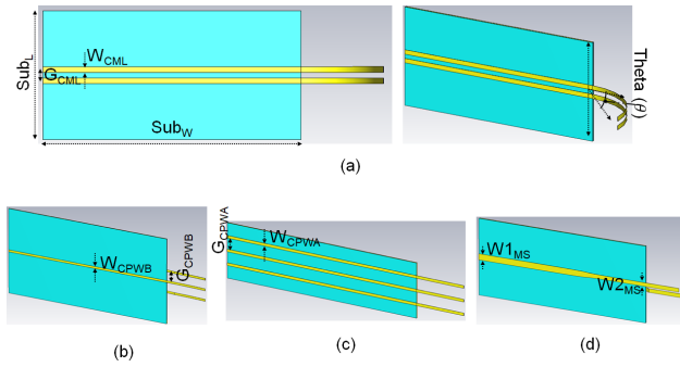
Figure 2: Investigated transition structures from active device (ZBSD) to IF circuit (a) Microstrip coupled lines, (b) Co-planar wave guide (CPW) as signal on top, (c) Co-planar wave guide (CPW) as all three ground-signal-ground on top and (d) Micro-strip line.
