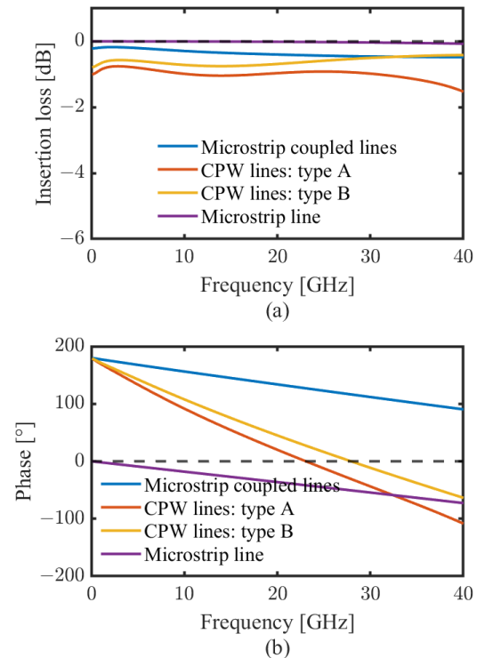
Figure 4: Comparison of different types of transition for a bending angle \theta is 0^\circ .
