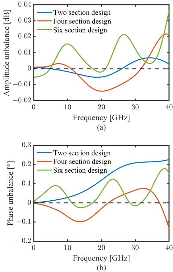
Figure 7: (a) Amplitude unbalance comparison for different sections and (b) Phase unbalance comparison for different sections.
